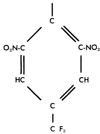
benefin
